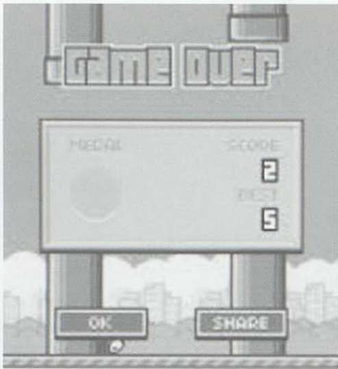
Flappy Bird
